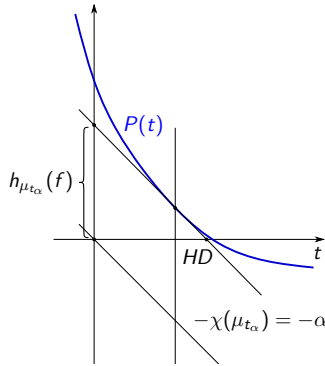
Figure 5. Legendre transform
